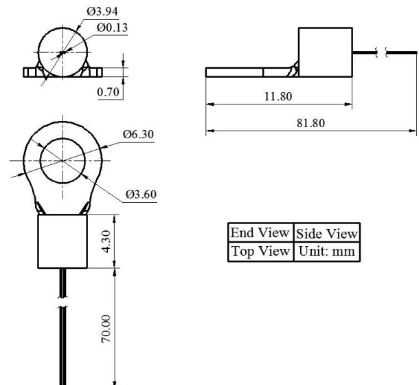
Figure 2. The Front and Side Views of ATH10KL2C
