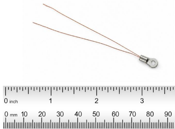
Figure 1.1. The physical photo of ATH10KL2B
