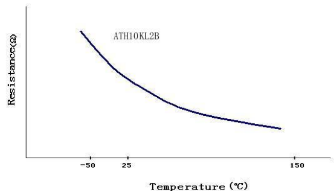
Figure 4. Resistance vs. Temperature for ATH10KL2B
