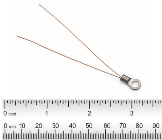
Figure 1.1. The physical photo of ATH100KL2C
