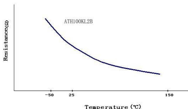
Figure 4. Resistance vs. Temperature for ATH100KL2B
