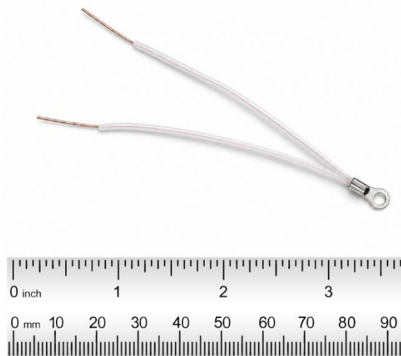
Figure 1.2. The physical photo of ATH100KL2BT70S
