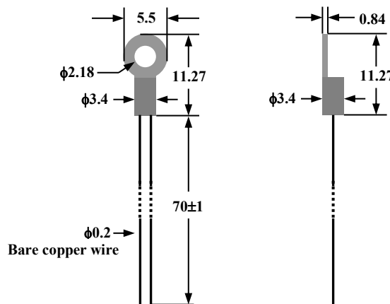
Figure 2. The Front and Side Views of ATH100KL2B
