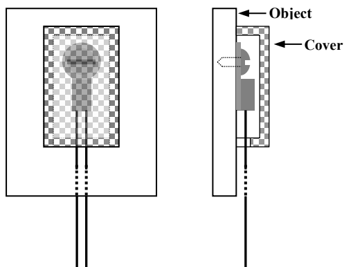
Figure 3. Using an Insulation Cover to Improve Accuracy
