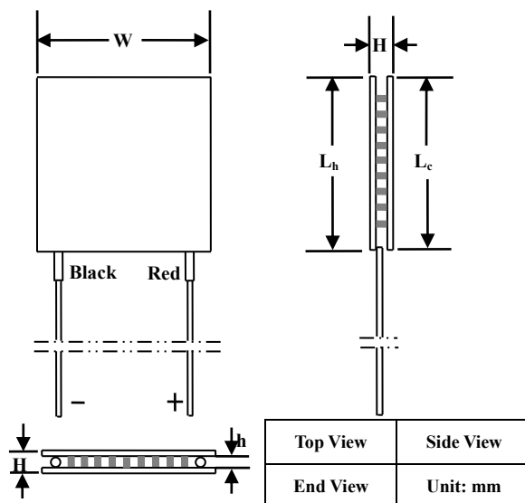
Figure 13. Mechanical Dimensions of Non-sealed ATE1-TCHE-32
