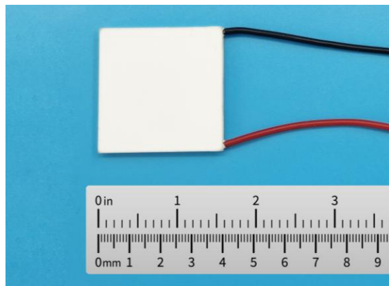
Figure 1. The Photo of Actual ATE1-TCHE-127
