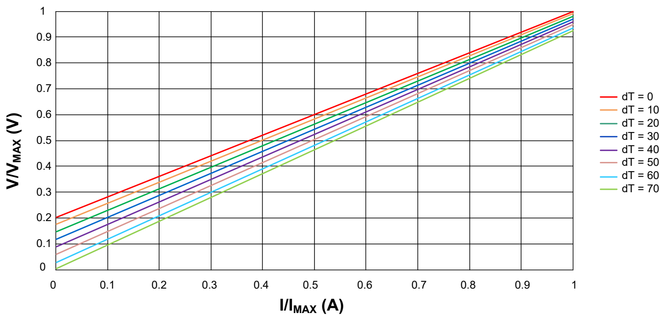
Figure 9. V / V_{MAX} vs. I / I_{MAX}
