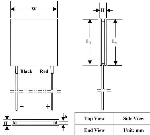
Figure 6. Mechanical Dimensions of ATE1-TC-31-3AS
