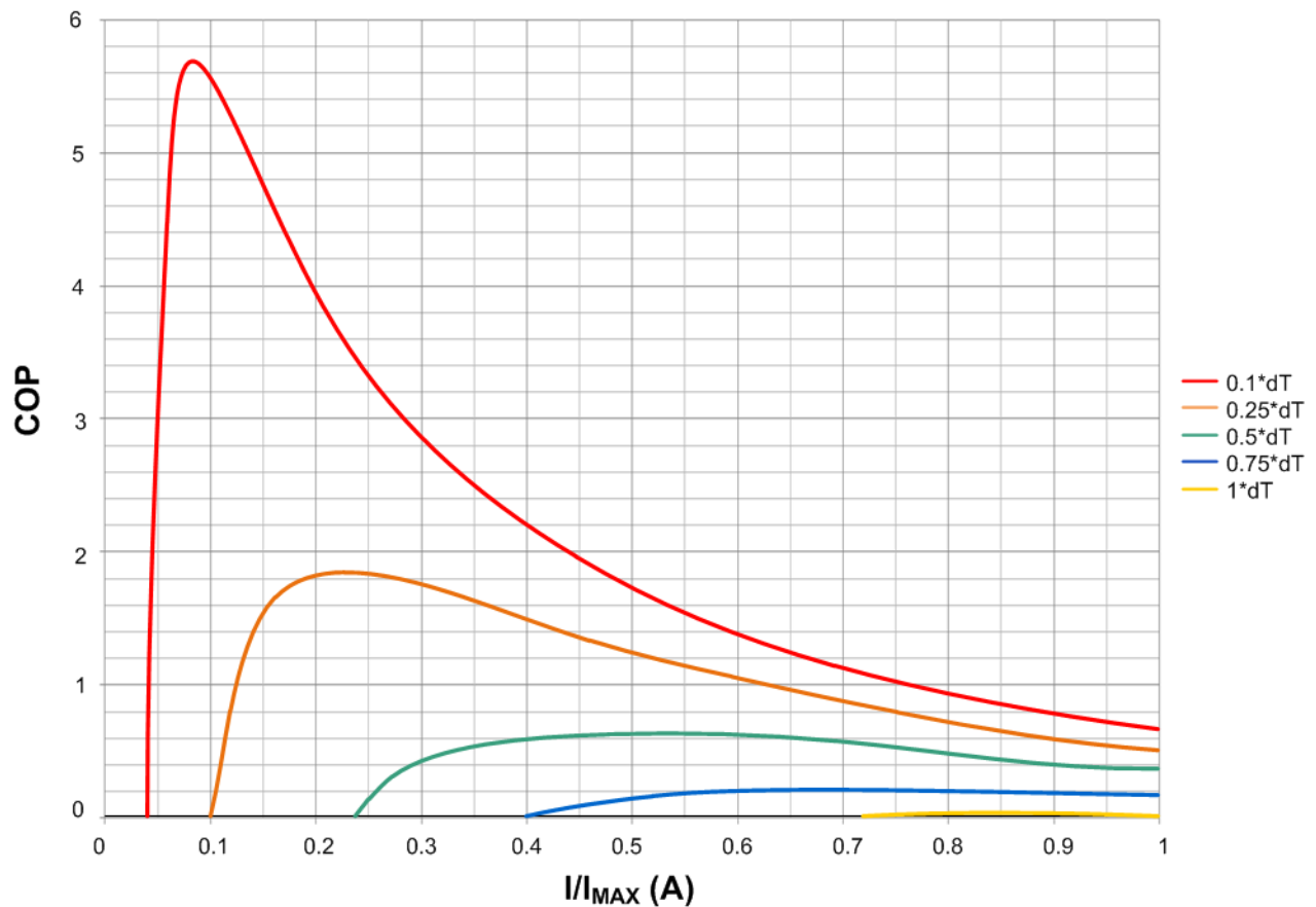
Figure 4. COP vs. dT_{MAX}
