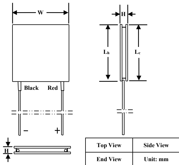
Figure 6. Mechanical Dimensions of Sealed TEC
