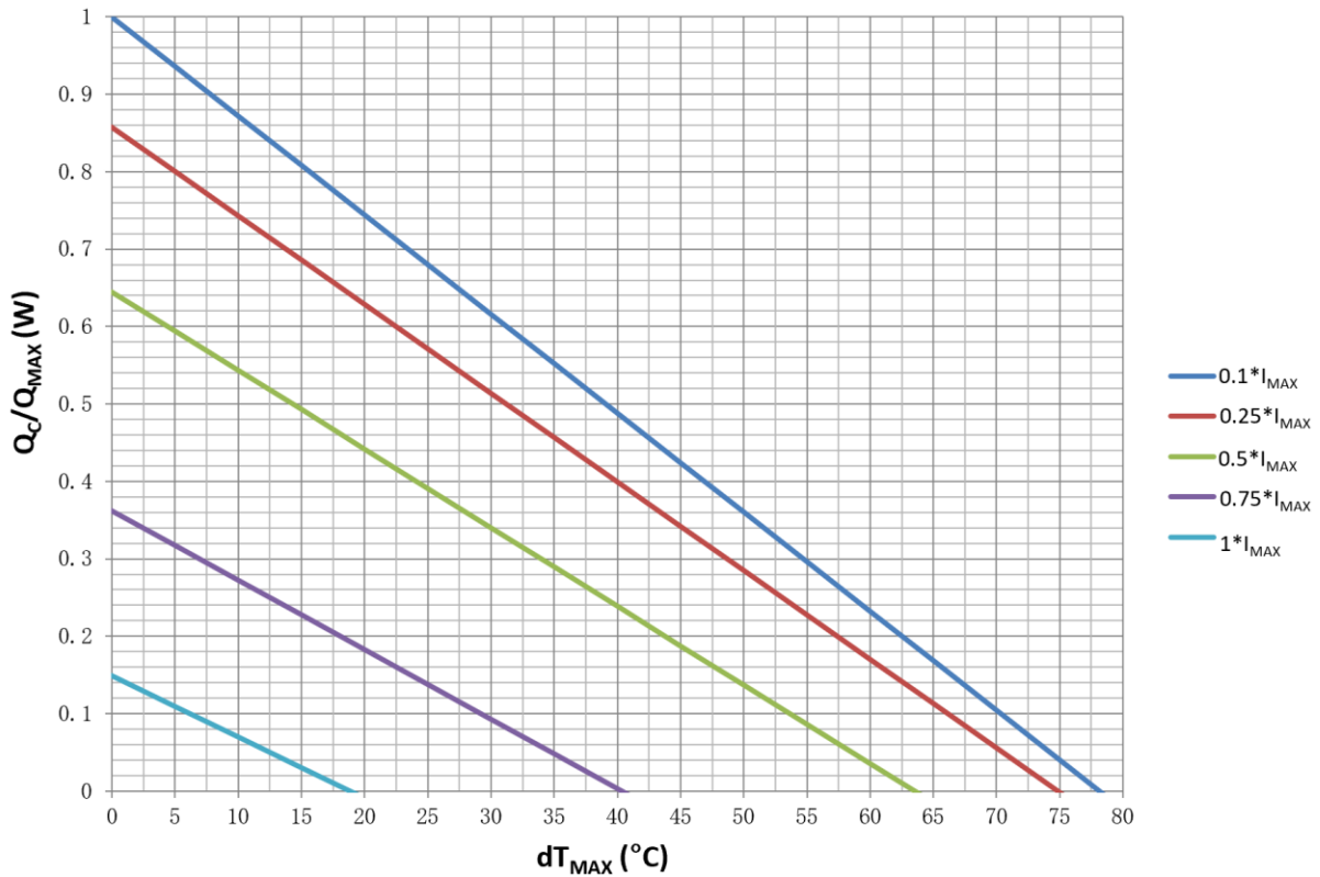
Figure 2. Q_c/Q_{MAX} vs. dT_{MAX}
