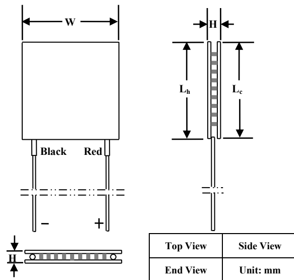
Figure 7. Mechanical Dimensions of Non-sealed TEC
