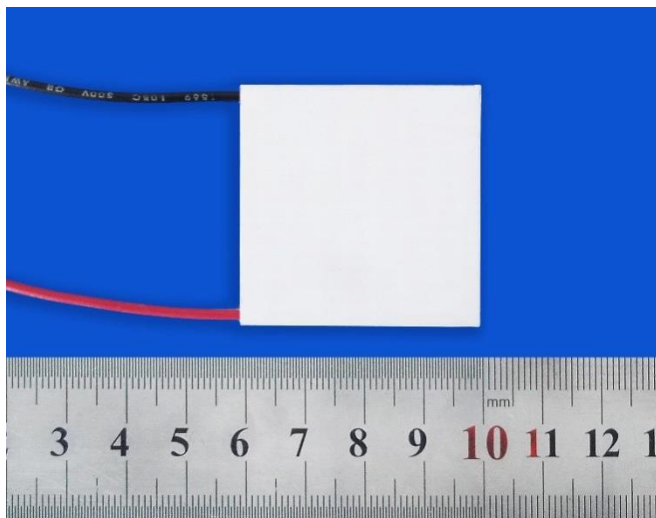
Figure 1. The Photo of Actual ATE1-TC-127-5R7A
