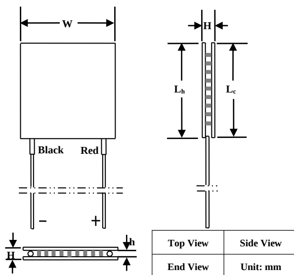
Figure 6. Mechanical Dimensions of Non-sealed ATE1-TC-127-5R7A
