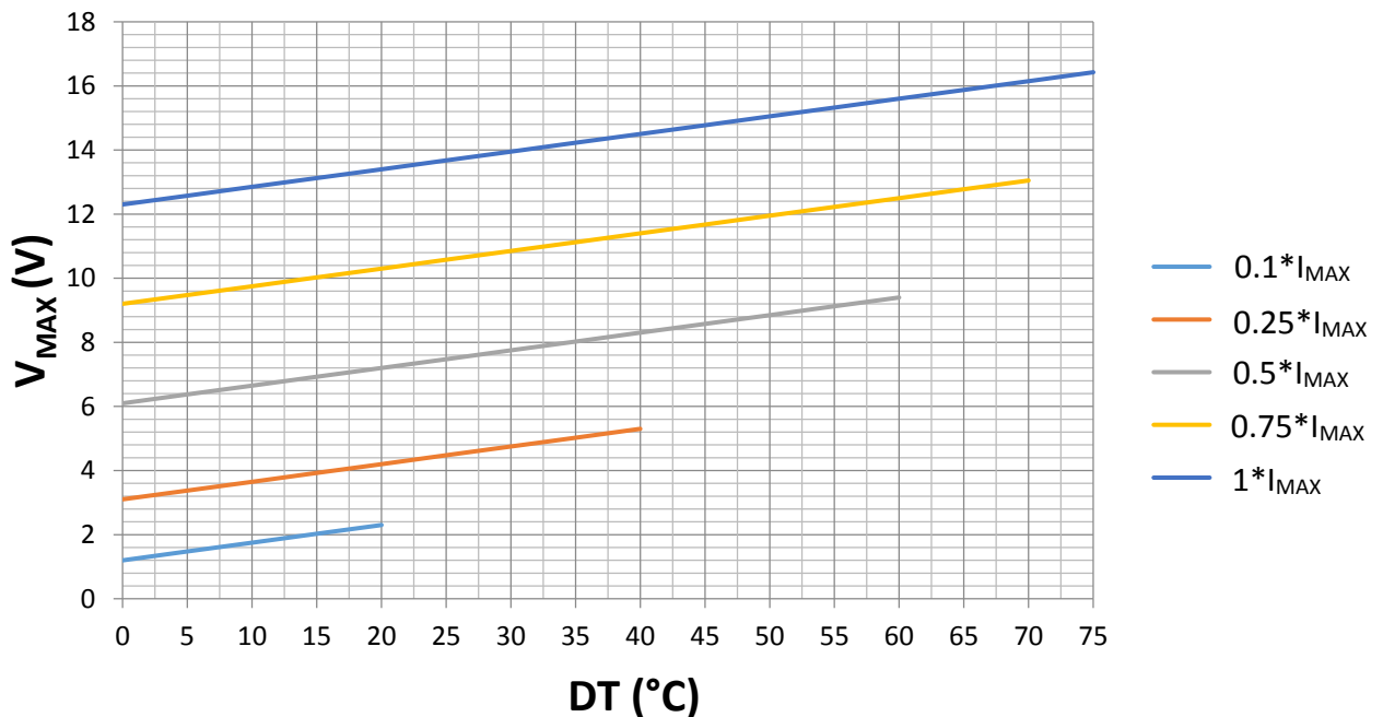
Figure 3. V_{MAX} vs. DT
