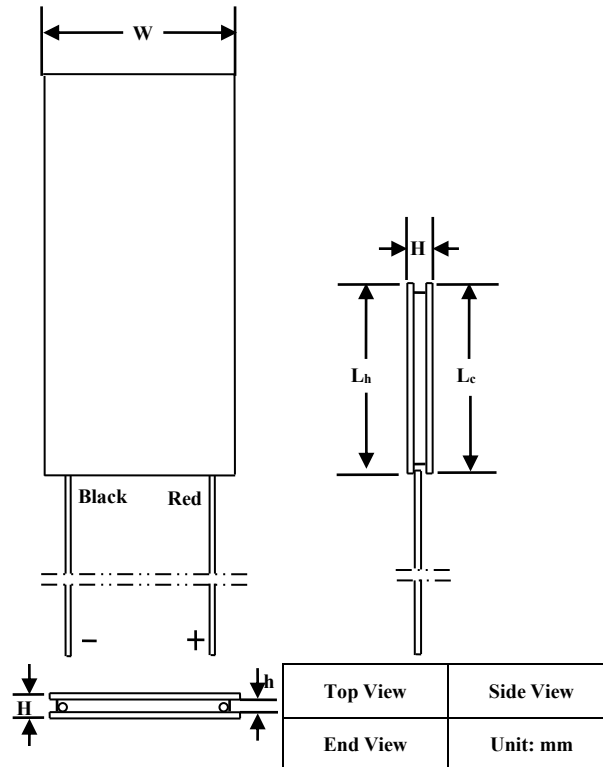
Figure 6. Mechanical Dimensions of Sealed ATE1-63
