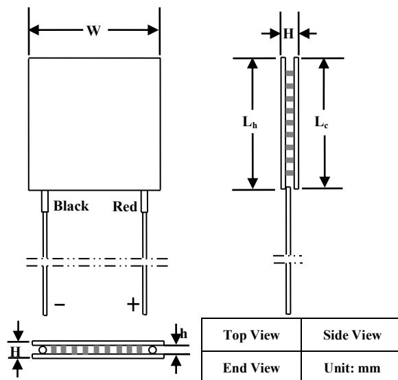
Figure 11. Mechanical Dimensions of Non-sealed ATE1-49
