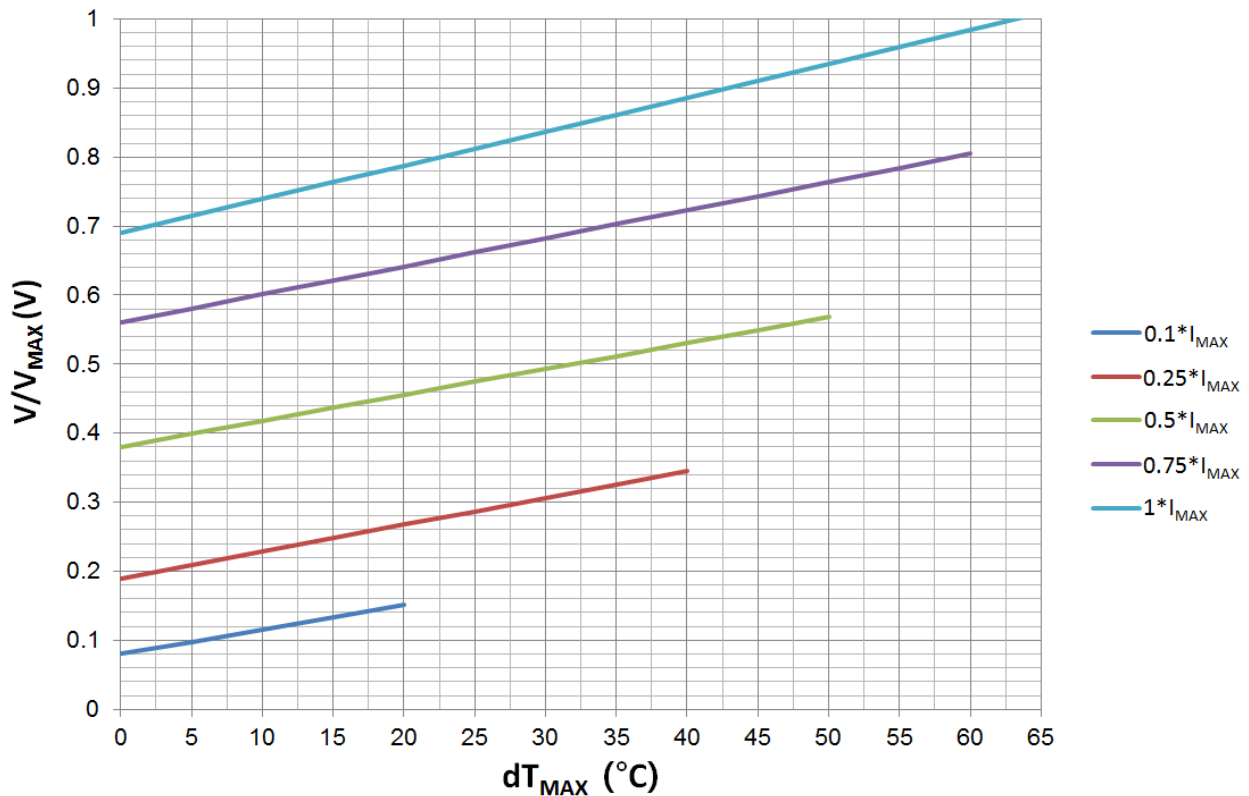
Figure 3. V/V_{MAX} vs. dT_{MAX}
