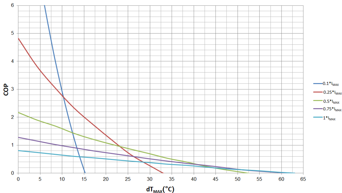
Figure 4. COP vs. dT_{MAX}
