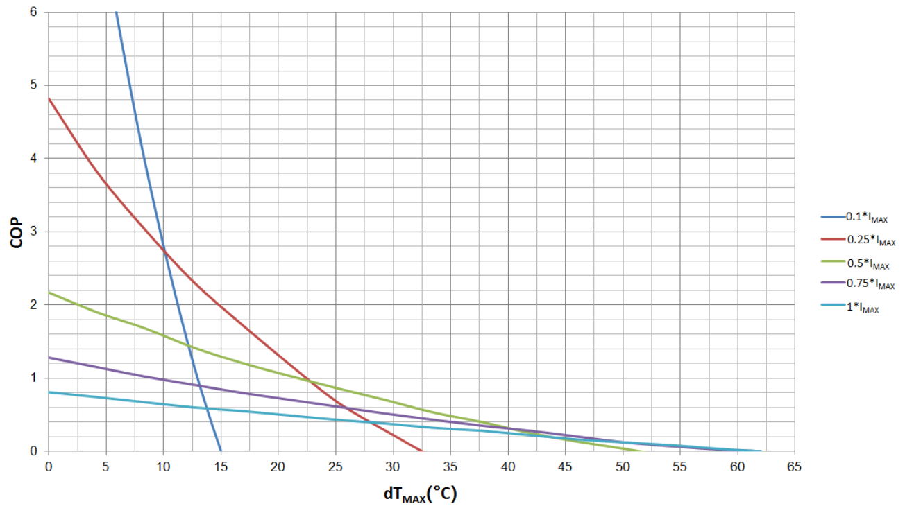
Figure 8. COP vs. dT_{MAX}
