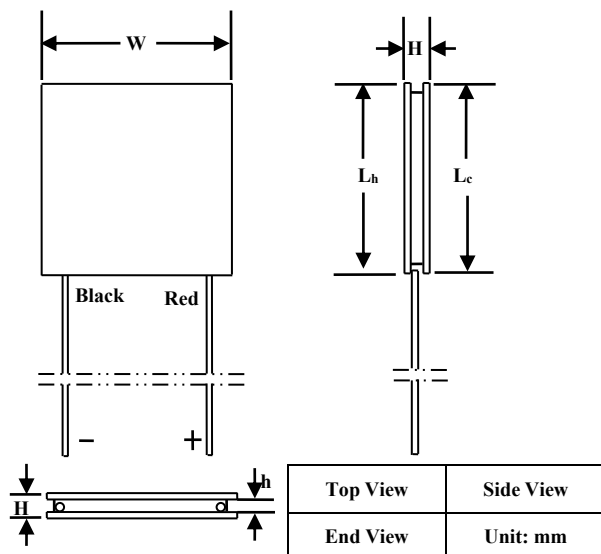
Figure 10. Mechanical Dimensions of Sealed ATE1-49
