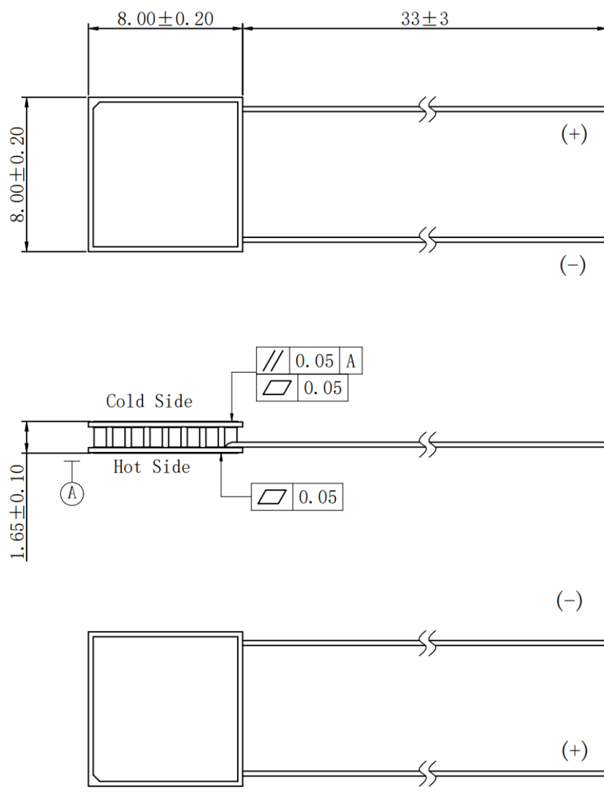
Figure 5. Mechanical Dimensions ATE1-31-2.4A-A
