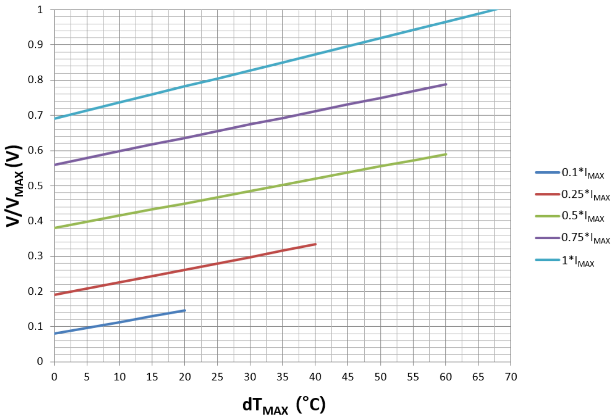
Figure 3. V/V_{max} vs. dT_{max}
