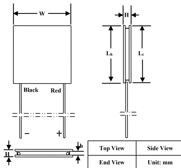
Figure 6. Mechanical Dimensions of ATE1-288
