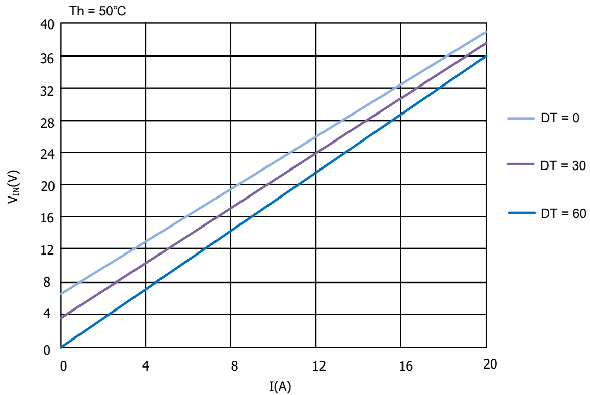
Figure 6. V_{IN} vs. I
