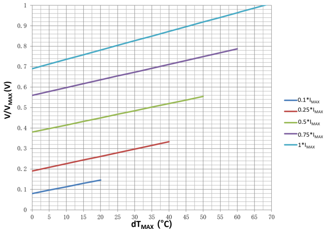
Figure 3. V/V_{MAX} vs. dT_{MAX}
