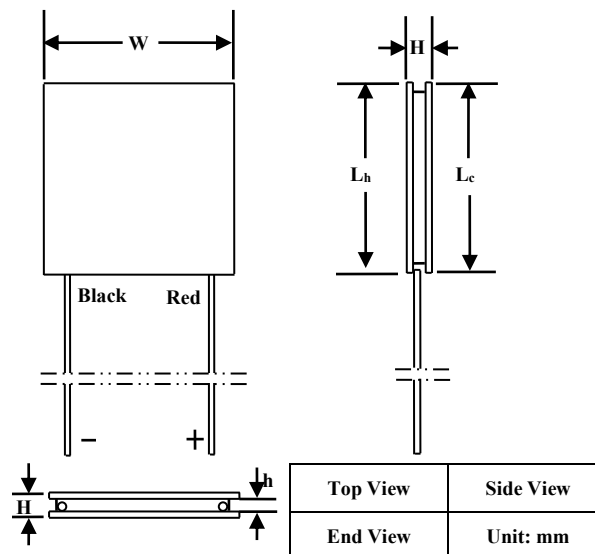
Figure 6. Mechanical Dimensions of ATE1-241
