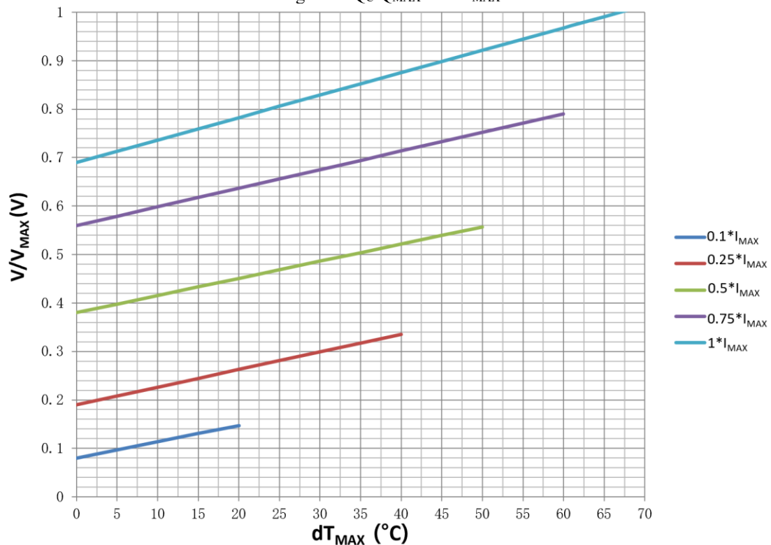
Figure 3. V/V_{MAX} vs. dT_{MAX}
