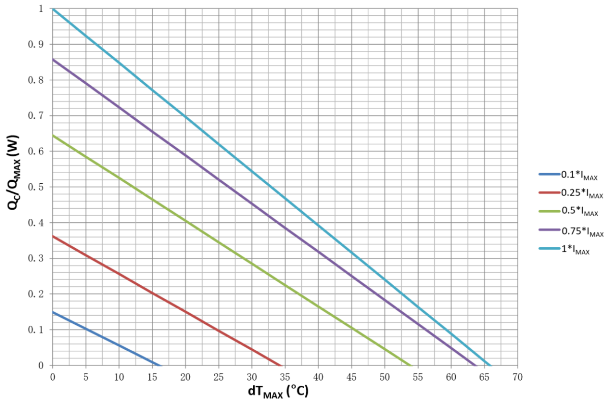
Figure 10. Q_C/Q_{MAX} vs. dT_{MAX}
