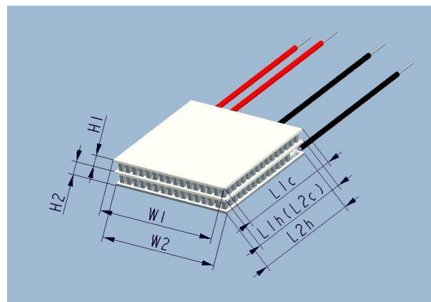
Two stages TEC Module (Non-sealed)
