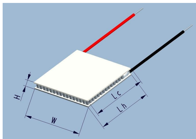
Single stage TEC Module (Non-sealed)
