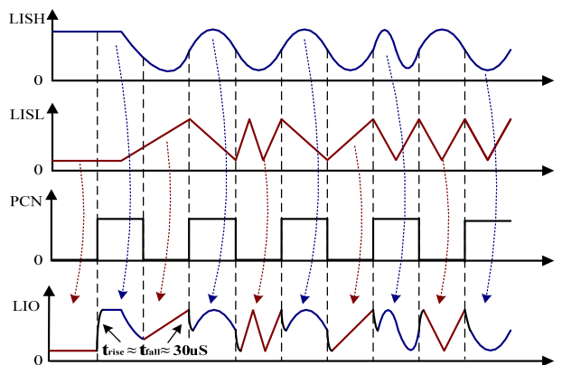
Figure 10. Digitally Controlled Analog Modulation Principle
