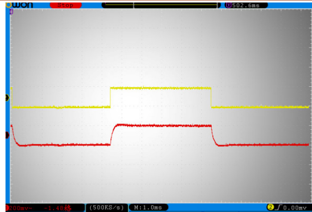
Figure 12. Small Signal Modulation
