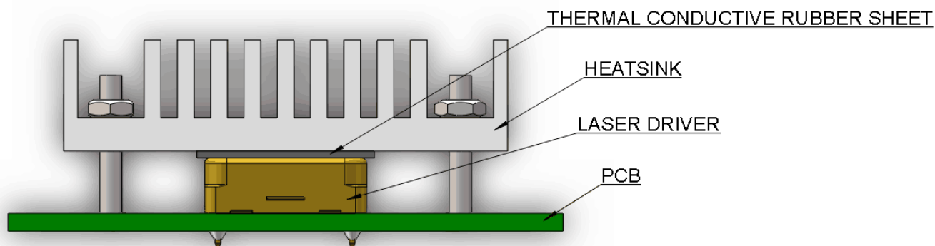
Figure 11.2 Transferring Heat with Heat Sink
