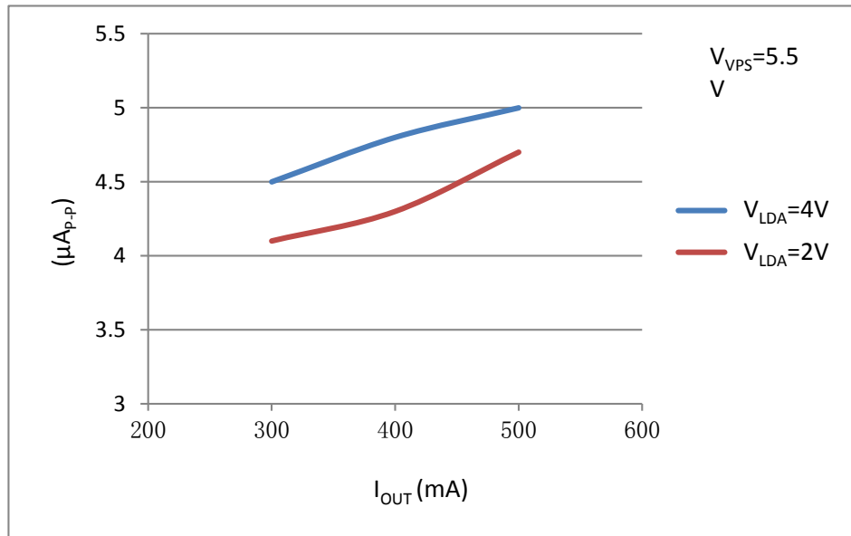
Figure 17. I_{OUT} vs. Output Current Noise@0.1Hz~10Hz
