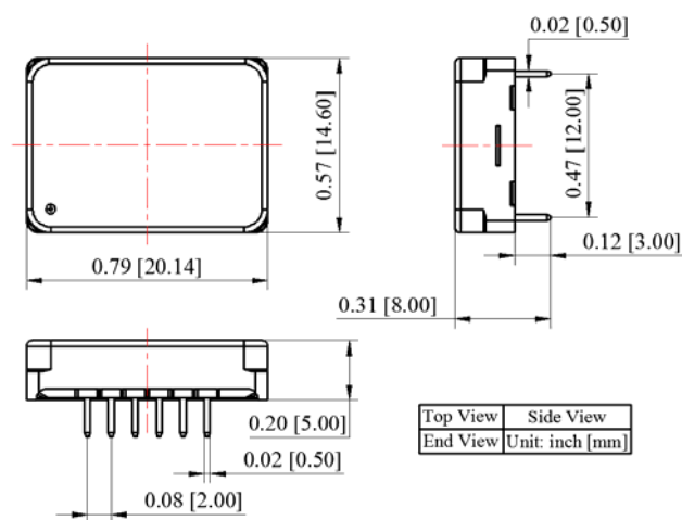
Figure 21. Dimensions of the DIP Package Controller
