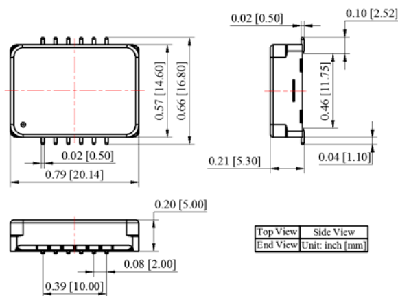
Figure 22. Dimensions of the SMT Package Controller
