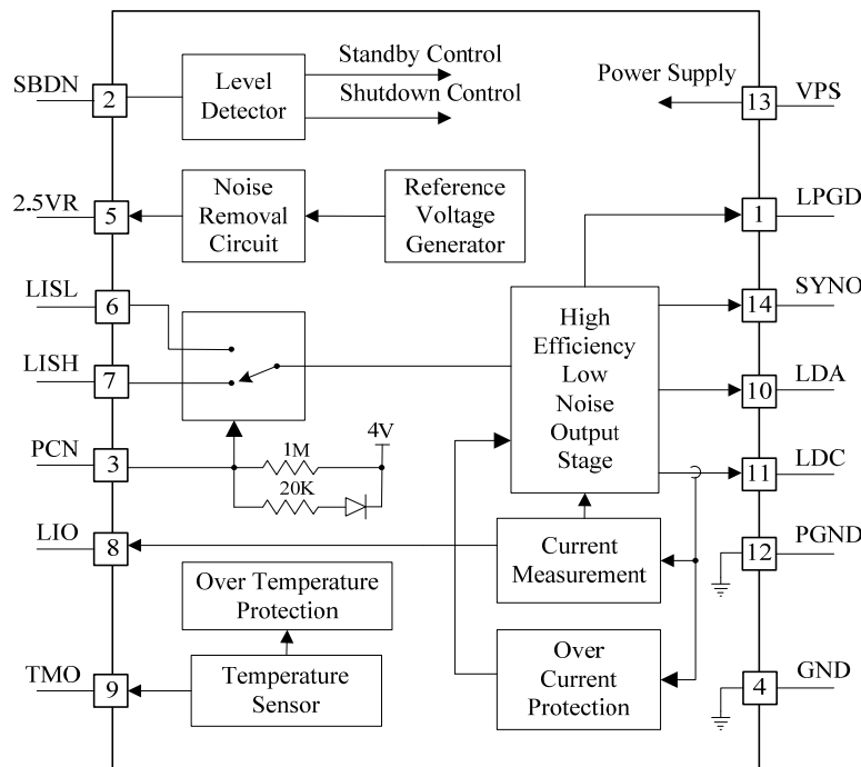
Figure 3. Internal Block Diagram of ATLS2A212
