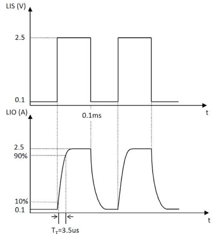
Figure 9. Large Signal Modulation
