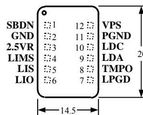
Figure 2. Pin Names and Locations
