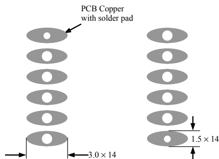
Figure 14. Top View of the Bottom Side PCB Foot-print
