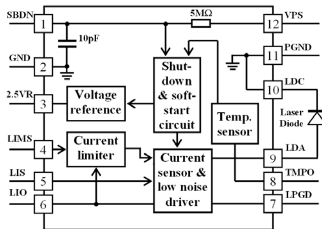
Figure 3. Block Diagram
