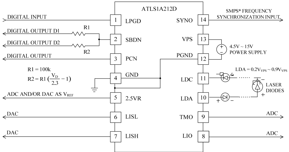
Figure 7. A Typical Micro-processor-based Application Schematic
