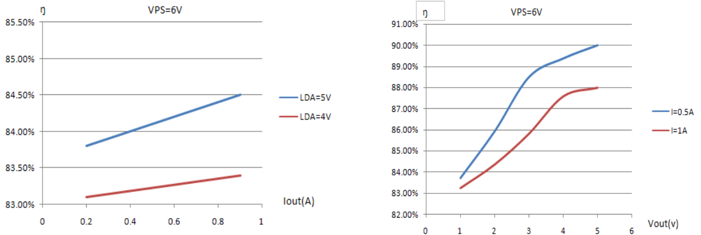
Figure12. Efficiency of Laser Driver
