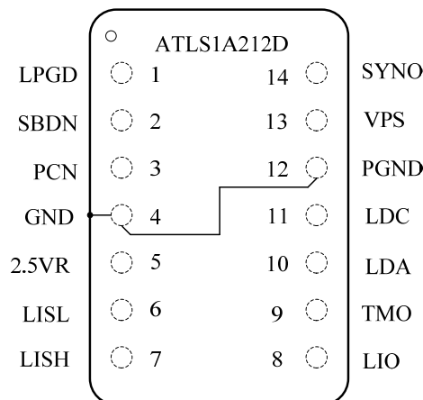
Figure 2. Pin Names and Locations
