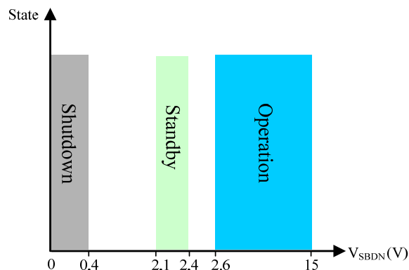
Figure 4. Input Control
