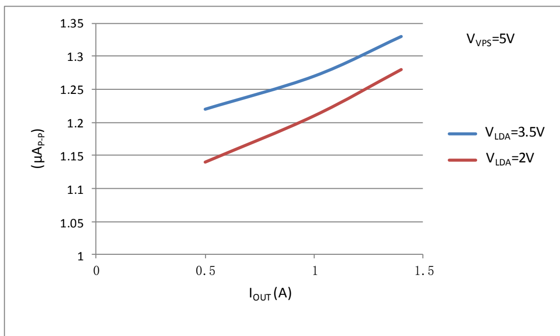
Figure 11.2. I_{OUT} vs. Output Current Noise@0.1Hz~10Hz
