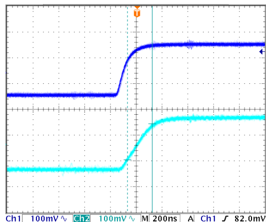
Figure 12.3. Small Signal Rise Time 192ns
