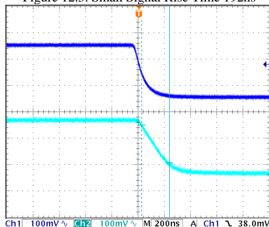
Figure 12.4. Small Signal Fall Time 212ns
