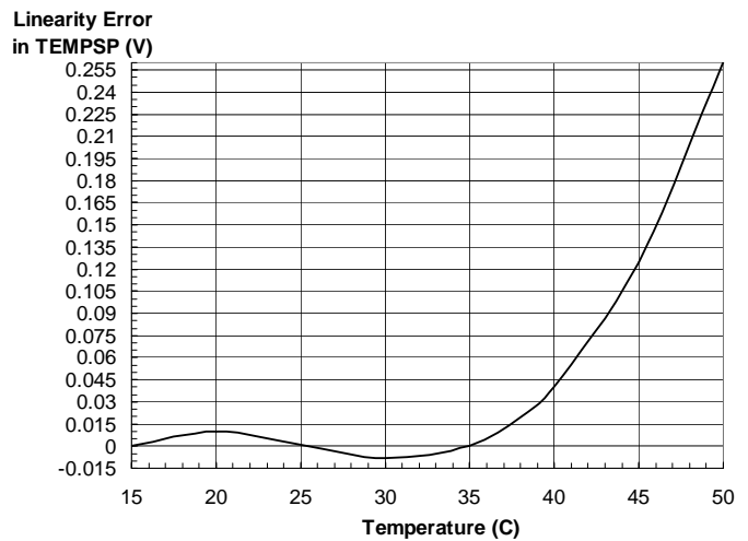
Figure 10 Linearity error in TEMPSP vs. Temperature
