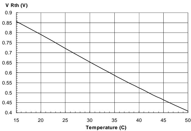
Figure 8 V_{Rth} vs. Temperature
