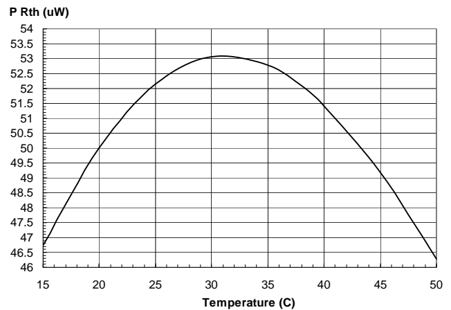
Figure 9 P_{Rth} vs. Temperature
