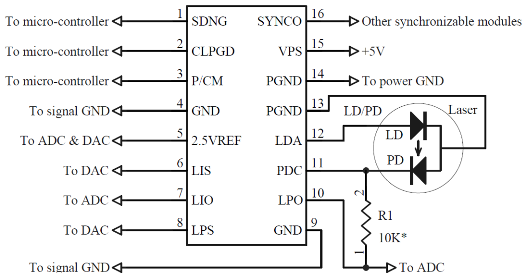
Figure 5 A Typical Micro-processor Based Application
